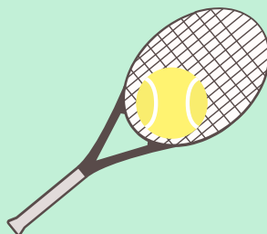
le tennis
